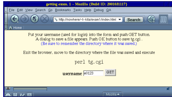
Figure 5: Get exam
